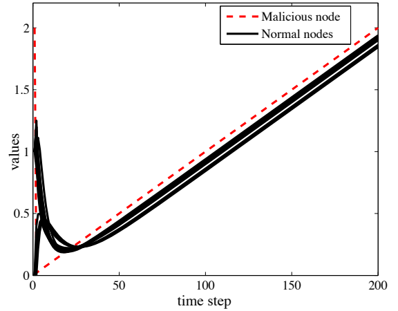
(a) LCP.
