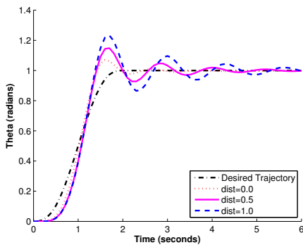
Figure 9. Joint 1 response ( T_s = .05 , \epsilon = 1.0e-6 , d = \{0, 0.5, 1.0\} ).
