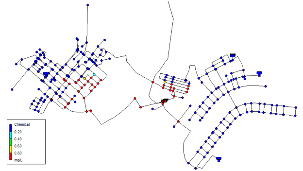
Figure 1: Topology of the water-distribution network. Colors show the spread of the chemical contaminant from the first reservoir two hours after its introduction.
