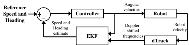
Figure 2: The robot navigation system.
