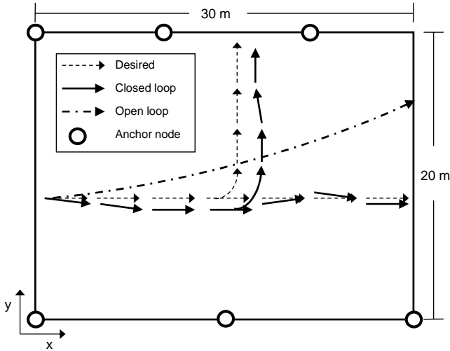
Figure 6: Robot trajectory under both closed-loop and open-loop experiments.
