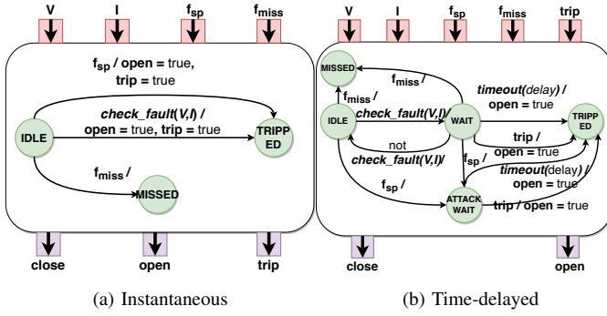
Fig. 3: Relay Elements
