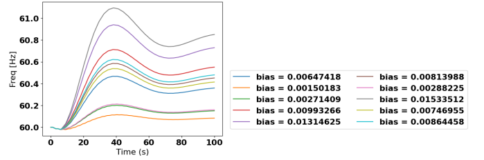
Fig. 5: Effect of multiple biasing attacks on system frequency
