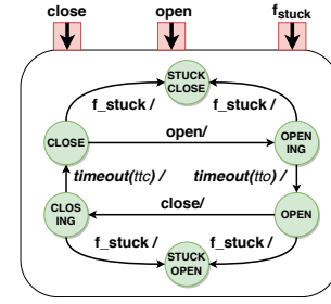
Fig. 4: Breaker Automaton
