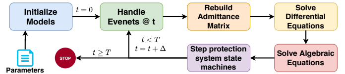
Fig. 2: Simulation Loop
