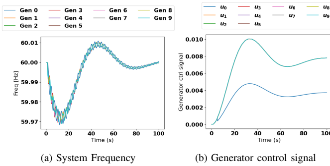
Fig. 6: Effect of scaling attack
