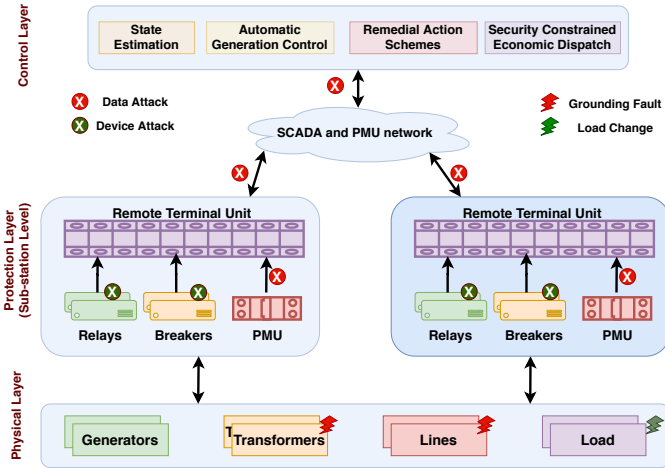
Fig. 1: Power-Attack tool-chain capabilities
