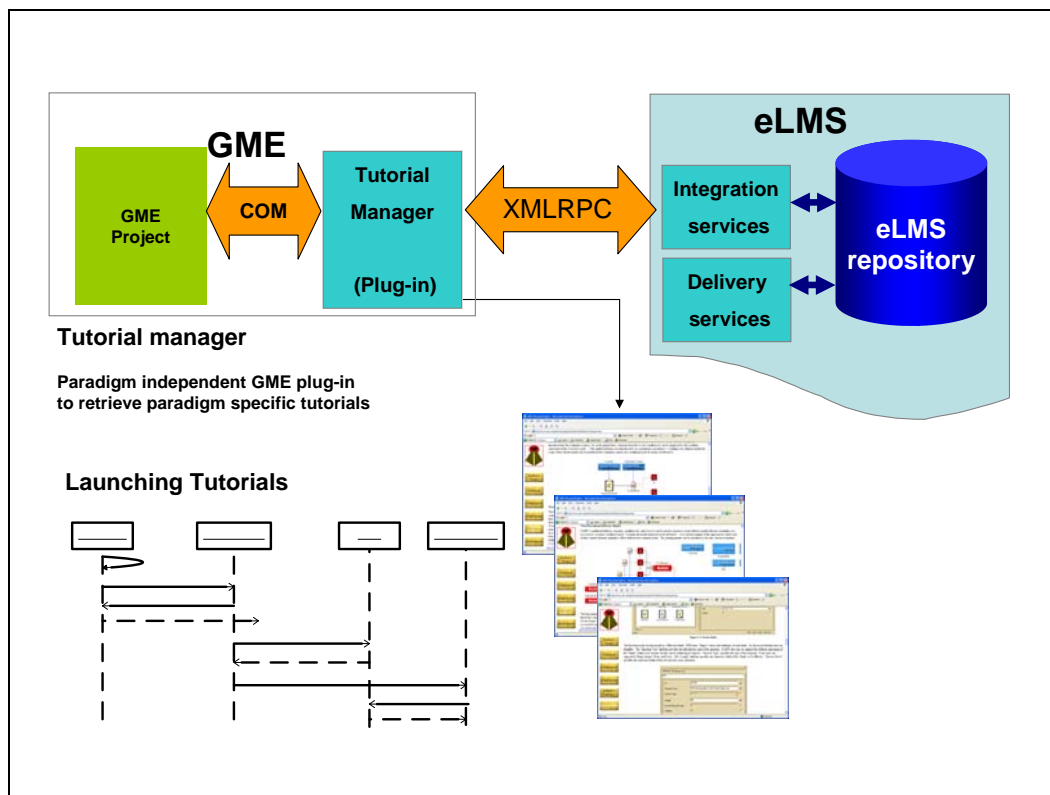
Figure 3: Tutorial Manager in GME
