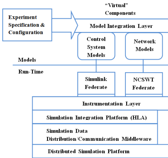
Figure 1: NCSWT Simulation Architecture
