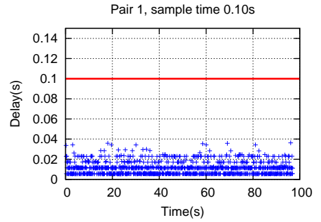
(a) Delay plot for P1-C1 pair
