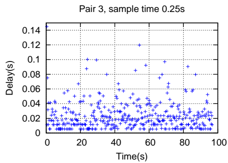
(c) Delay plot for P3-C3 pair
