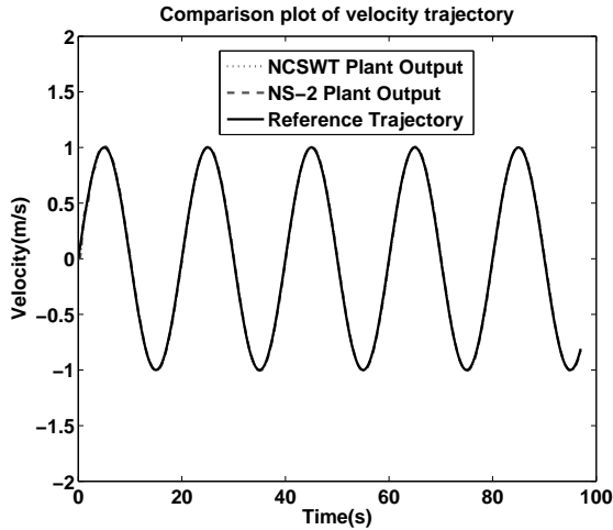
Figure 5: Comparison plot of velocity trajectory.
