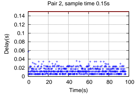
(b) Delay plot for P2-C2 pair
