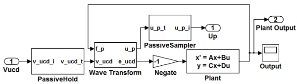
Figure 13: Simulink model of simple plant node.
