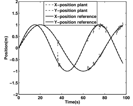
(a) Output plot for 20% loss rate.
