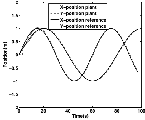
(b) Output plot for Five hops.
