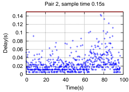
(b) Delay plot for P2-C2 pair
