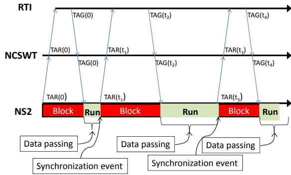
Figure 3: Time synchronization between the ns-2 and the RTI
