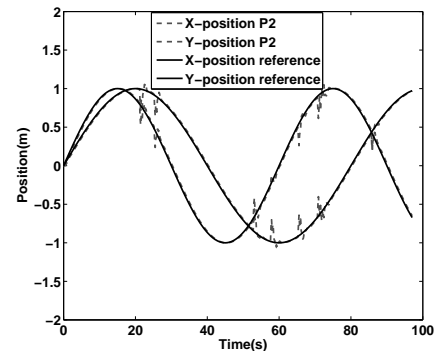
(b) Output plot for Plant P2.
