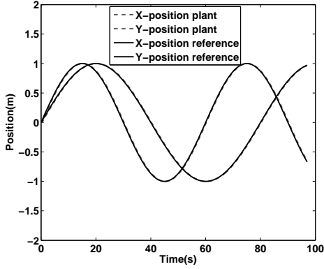
Figure 7: Plant Output for Nominal Case.
