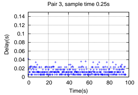
(c) Delay plot for P3-C3 pair
