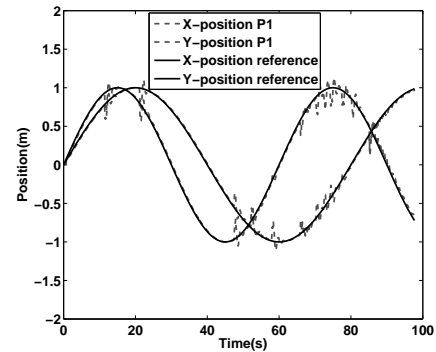
(a) Output plot for Plant P1.
