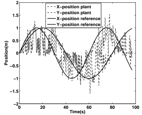
(b) Output plot for 40% loss rate.
