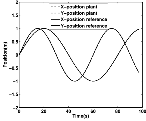
(a) Output plot for Three hops.
