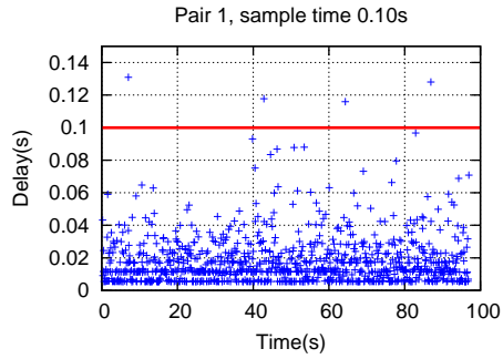
(a) Delay plot for P1-C1 pair
