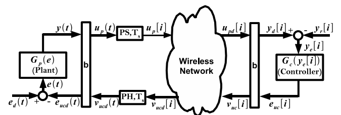
Figure 4: Passivity Based Control Architecture for a Single Plant System and a Single Controller Over Wireless Networks
