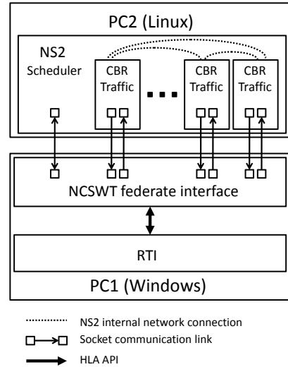
Figure 2: NCSWT communication overview
