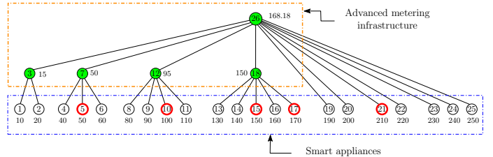
Fig. 1. A building area network represented by a tree graph.
