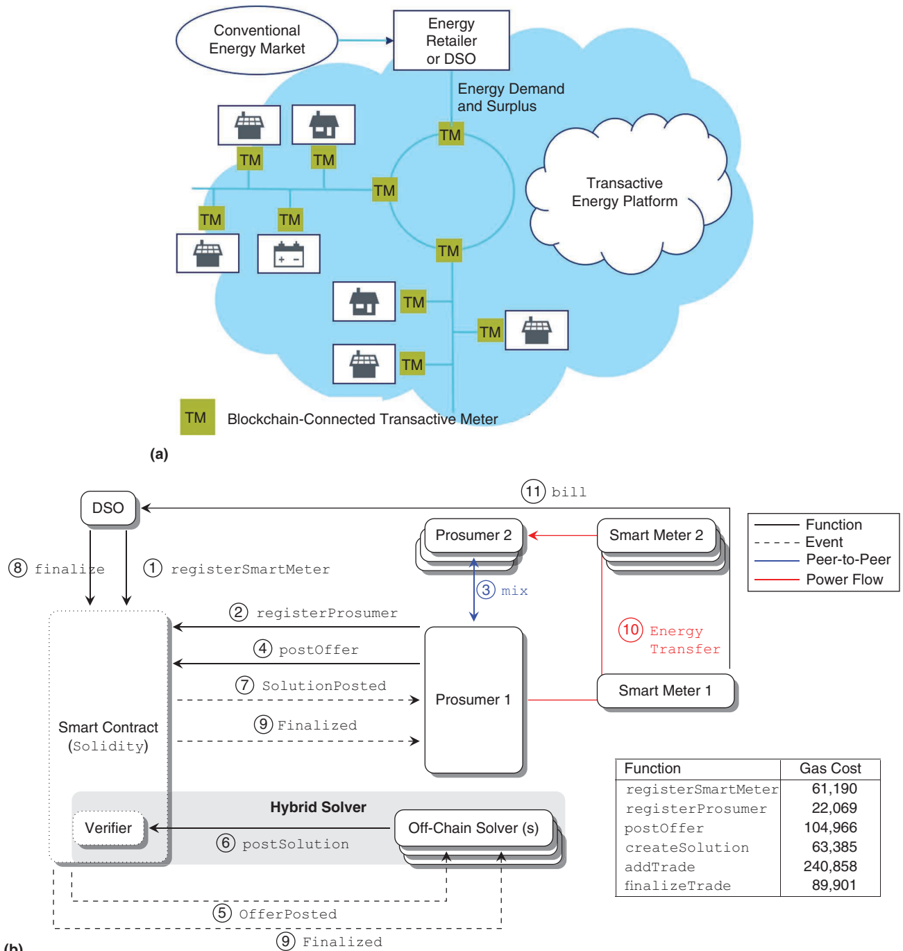
FIGURE 1. (a) The physical microgrid topology in TRANSAX. Every node is managed by a smart meter, which has access to the blockchain and ensures proper billing per node. (b) The information architecture of TRANSAX and the control flow of the interaction between components. The gas costs for each function were estimated using the Remix editor and are shown in the inset table. The postSolution is a composite function that requires the solver to call createSolution followed by a number of addTrade invocations. Each addTrade specifies a seller, a consumer, the time interval, and the energy to be transferred. The function finalize is invoked a few intervals (can be configured) before the interval being finalized. The finalize call also requires the smart contract to check each trade that is part of that interval. The cost of single-trade finalization is shown in the inset table. This cost is paid for each finalized trade.
