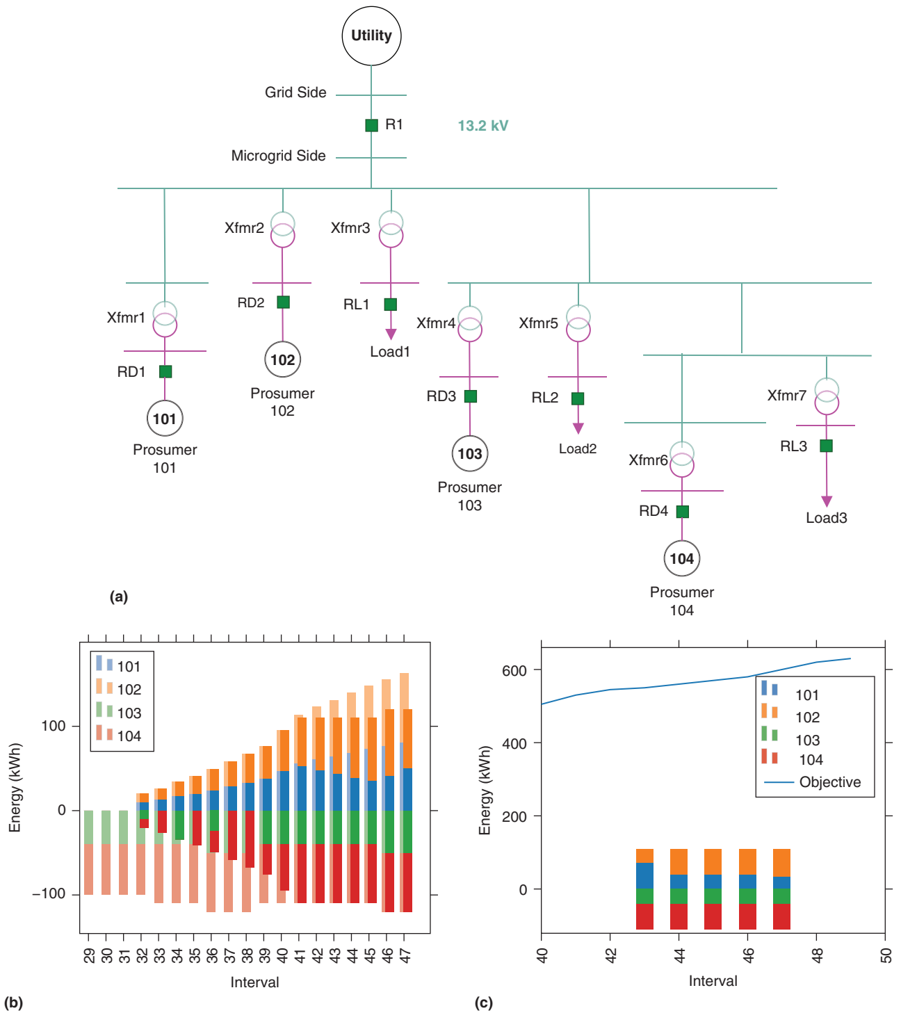
FIGURE 2. (a) The microgrid used in the case study. Prosumers 103 and 104 are consumers. Prosumers 101 and 102 produce energy. Other loads are passive and supplied by the utility. (b) The offers and subsequent trades made in the system. Lighter colors represent the offers that were made in an interval by a prosumer. Darker colors represent the actual trades that were matched and executed through TRANSAX in an interval. (c) The objective and trades for an interval evolve over time before the interval is finalized. Xfmr: transformer; R: resistor; L: inductor; D: diode.
