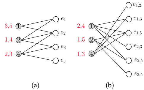
Fig. 2. Graph labelings for \mathcal{K} = \{1, 2, \dots, 5\} and \sigma = 2 . Node labels, i.e., f(x) are shown in red.
