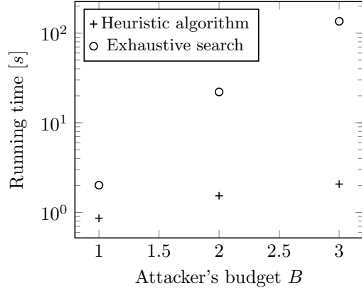
Figure 4: Running times of the heuristic algorithm and the exhaustive search, for randomly generated networks mimicking road networks of the USA.
